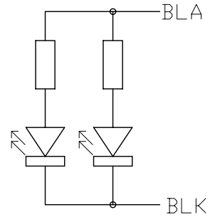
Backlight Circuit (No. of LEDs = 2pcs) Scale=free
