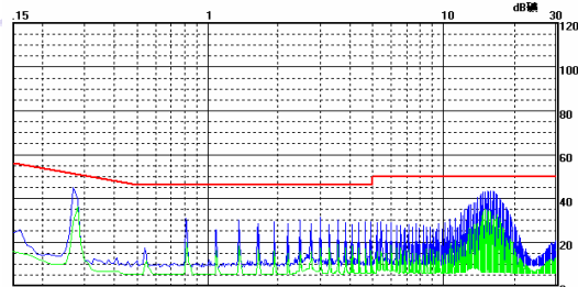
WRB1205S-3WR2 CE(Class B, Positive line)
