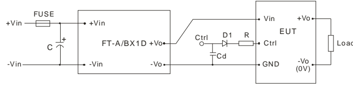
FT-A/BX1D is MORNSUN's EFT suppressor For Nominal Voltage < 48V, C \geq 330\mu\text{F}/50\text{V} For Nominal Voltage = 48V, C \geq 330\mu\text{F}/100\text{V} (Figure 3)
