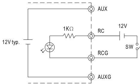
(C) Using internal 12V auxiliary output
