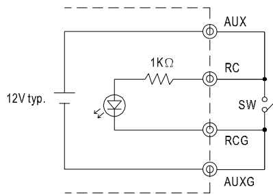
(C) Using internal 12V auxiliary output
