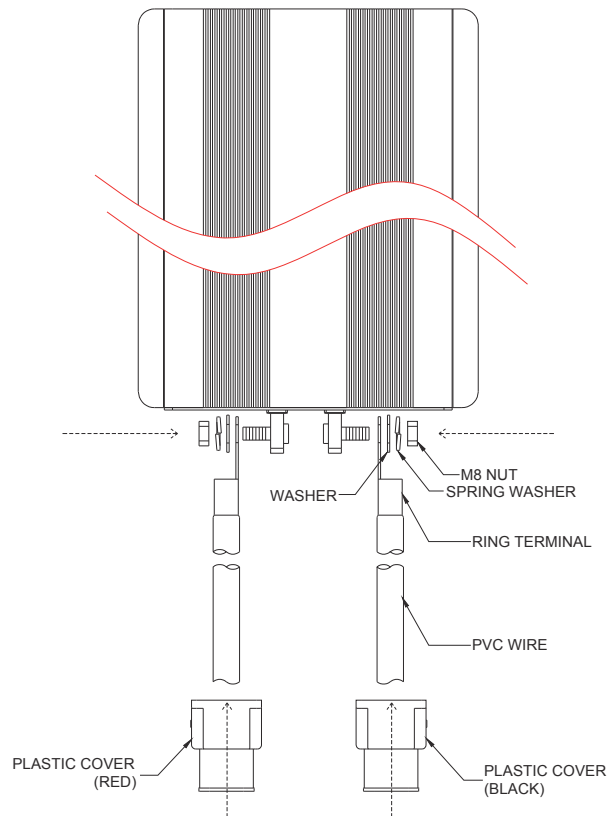
Battery to inverter cable connection
