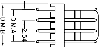
(2 through 5 circuits)
