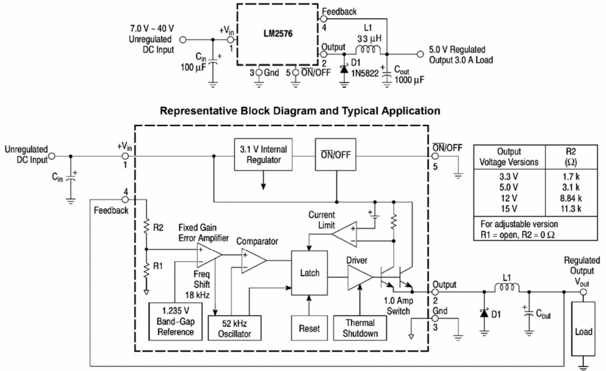
Figure 1. Block Diagram and Typical Application
