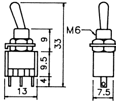
B068EPB 6P MINIATURE TOGGLE SWITCH (DPDT) ON-ON 120V 5A (250V 2A)
