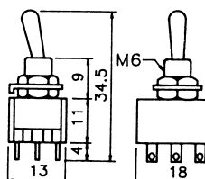
B068EW 6P MINIATURE TOGGLE SWITCH (DPDT) ON-ON 120V 5A (250V 2A)
