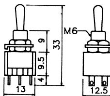
B068BW 3P MINIATURE TOGGLE SWITCH (SPDT) ON-ON 120V 5A (250V 2A)
