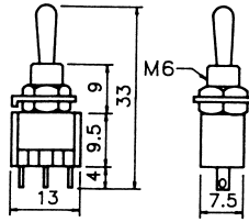
B068BV 3P MINIATURE TOGGLE SWITCH (SPDT) ON-ON 120V 5A (250V 2A)
