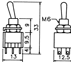
B068EV 6P MINIATURE TOGGLE SWITCH (DPDT) ON-ON 120V 5A (250V 2A)
