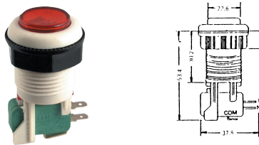
B181L PUSHBUTTON SWITCH (SPDT) ON-ON 250V 5A
