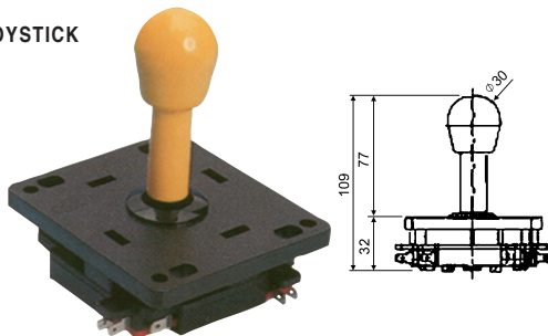
B182D OMNIPOTENT JOYSTICK ON-OFF 12V 1A
