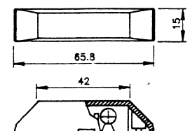
B182S (B1958) REED-ALARM SWITCH NC TYPE DOUBLE-DECK SHELL TO CIONCEAL SCREW HOLD OPERATING GAP 3.2cm MAX
