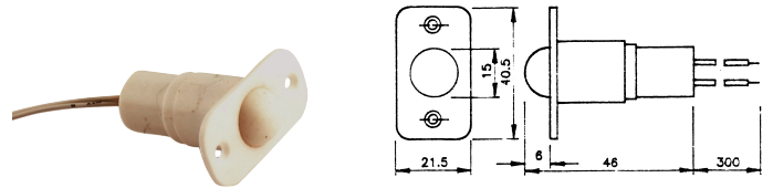
B182G (B1950) REED-ALARM SWITCH PUSH ON TYPE OPERATING GAP 3.5mm MAX
