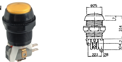
B181M ILLUMINATED PUSHBUTTON SWITCH W/O LAMP (SPDT) ON-ON 12V 1A
