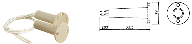
B182J (B1952) REED-ALARM SWITCH NC TYPE OPERATING GAP 2.3cm MAX
