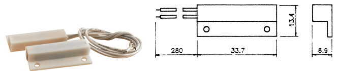
B182J (B1952) REED-ALARM SWITCH NC TYPE OPERATING GAP 2.3cm MAX
