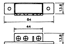
B182N (B1955) REED-ALARM SWITCH NO TYPE OPERATING GAP 3cm MAX
