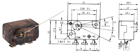
B182G (B1950) REED-ALARM SWITCH PUSH ON TYPE OPERATING GAP 3.5mm MAX
