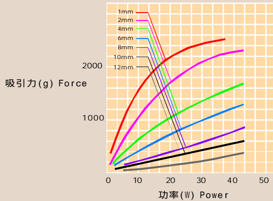
功率/吸引力 Power and Force
