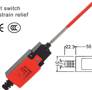
B18445H Safety limit switch W/rubber strain relief
