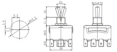
KN3C-402P ON-ON KN3C-403P ON-OFF-ON 4PDT 12P
