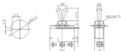
KN3B-102 ON-ON KN3B-112 ON-(ON) KN3B-103 ON-OFF-ON KN3B-113 ON-OFF-(ON) KN3B-123 (ON)-OFF-(ON) SPDT 3P
