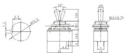
KN3-1 ON-OFF SPST 2P 4A 125VAC; 2A 250VAC
