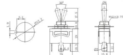
KN3C-102P ON-ON KN3C-112P ON-(ON) KN3C-103P ON-OFF-ON KN3C-113P ON-OFF-(ON) KN3C-123P (ON)-OFF-(ON) SPDT 3P
