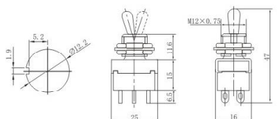
KN3-3A ON-ON DPDT 6P 6A 125VAC; 3A 250VAC
