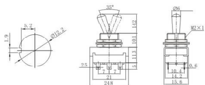
KN-32 ON-ON DPDT 6P 10A 125VAC; 5A 250VAC
