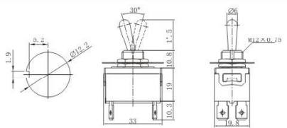
KN3C-201P ON-OFF KN3C-211P OFF-(ON) DPST 4P
