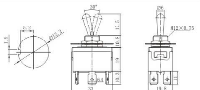
KN3C-202P ON-ON KN3C-212P ON-(ON) KN3C-203P ON-OFF-ON KN3C-213P ON-OFF-(ON) KN3C-223P (ON)-OFF-(ON) DPDT 6P
