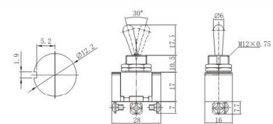
KN3A-102 ON-ON KN3A-112 ON-(ON) KN3A-103 ON-OFF-ON KN3A-113 ON-OFF-(ON) KN3A-123 (ON)-OFF-(ON) SPDT 3P
