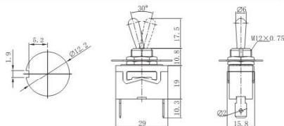
KN3C-101P ON-OFF KN3C-111P OFF-(ON) SPST 2P
