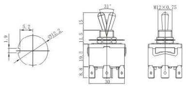
KN3C-302P ON-ON KN3C-303P ON-OFF-ON 3PDT 9P
