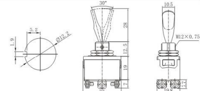
KN3C-202E ON-ON KN3C-212E ON-(ON) KN3C-203E ON-OFF-ON KN3C-213E ON-OFF-(ON) KN3C-223E (ON)-OFF-(ON) DPDT 6P
