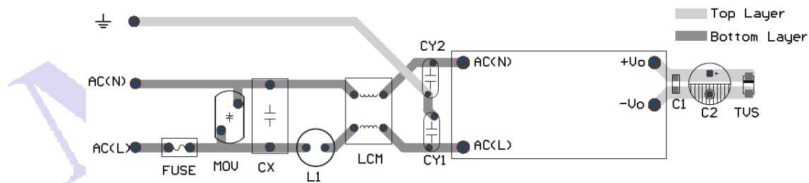
(figure 4): EMC application circuit PCB layout Safety and recommend wiring: linewidth \geq 3\text{mm} , line-line distance \geq 6\text{mm} , line- ground distance \geq 6\text{mm}
