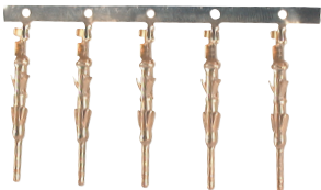
CRIMP TERMINAL GOLD PLATED PLUG : ZDVP35T (2500PINS / ROLL)
