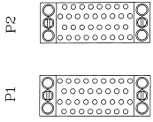
ZR0722 MM/MF DB25 TO V.35 CABLE (6ft) MM: DB25 MALE TO V.35 MALE MF: DB25 MALE TO V.35 FEMALE
