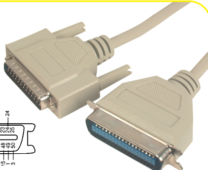
ZR15MM SCSI I TO SCSI II CABLE ( 3ft ) MM : HPC50M - CEN50M
