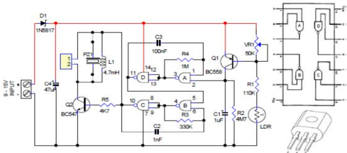
SCHEMATIC
