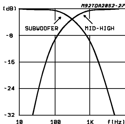
Figure 19: Frequency Response
