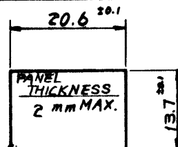
MOUNTING HOLE DETAIL (SCALE 1:1)
