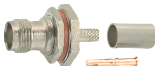
M5756 TNC female crimp type gold-pin (RG58U/59U)
