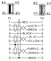
ZR07007 USB 3.0/A type plug to USB 3.0/A type jack cable (6ft)
