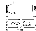
ZR07018 USB/A type plug to 5P micro USB/B type plug cable (6ft)
