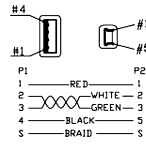
ZR07016 USB/A type plug to 5P mini USB/B type plug cable (6ft)
