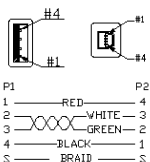
ZR07015 USB/A type plug to 4P mini USB/A type plug cable (6ft)
