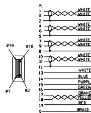
ZR07026 19P HDMI male to 19P HDMI male cable (6ft)
