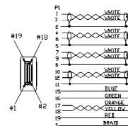
ZR07025 DVI 24+1 digital male to 19P HDMI male cable (6ft)
