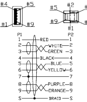
ZR07009 USB 3.0/A type plug to USB 3.0/B type plug cable (6ft)
