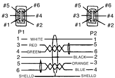
ZR07010 IEEE 1394 6P plug to 6P plug cable (6ft)
