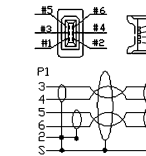
ZR07022 IEEE 1394 4P plug to IEEE 1394 6P plug cable (6ft)
