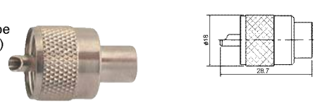
M5521 UHF male twist on type (RG58U/59U)
