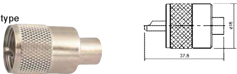
M5502 UHF male twist on type (RG8AU)
