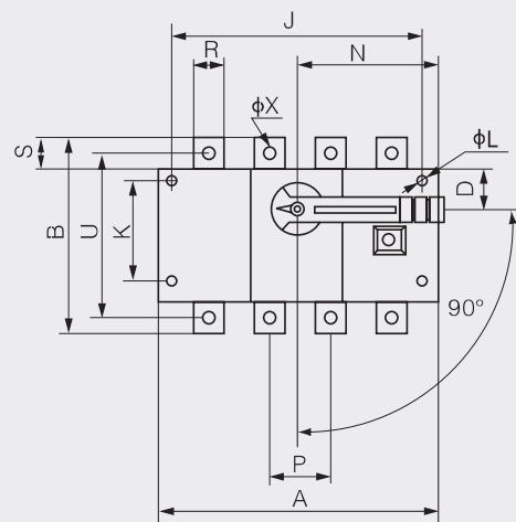
Direct operation of HGL-160A~630A
