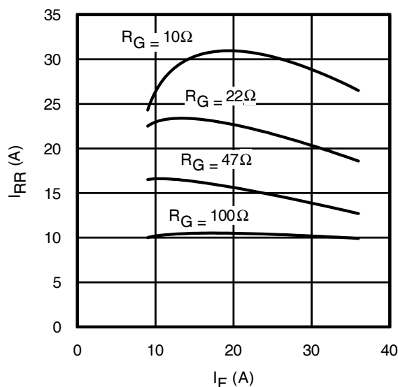
Fig. 18 - Typ. Diode I_{\text{RR}} vs. I_F
