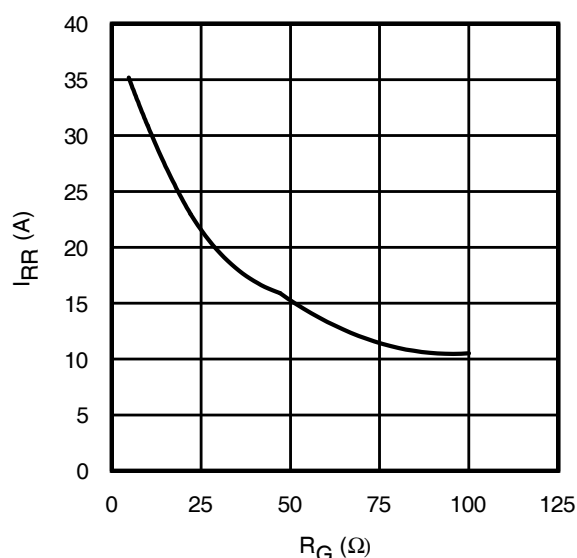
Fig. 19 - Typ. Diode I_{\text{RR}} vs. R_G
