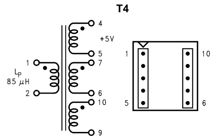
Figure 33. Coilcraft Q4344-B (Top View)
