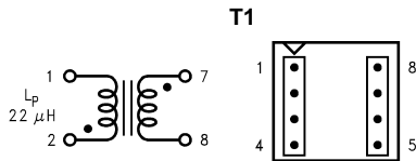
Figure 30. Coilcraft Q4434-B (Top View)
