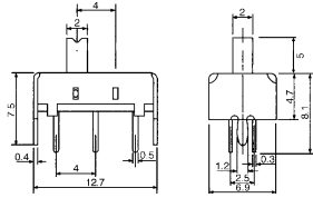
B1576 SLIDE SWITCH (2P3T)
