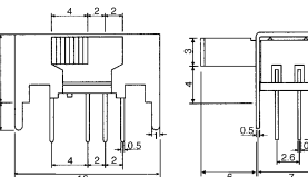
B15830 SLIDE SWITCH (6P3T)
