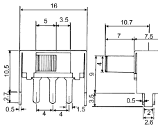
B15800 SLIDE SWITCH (4P2T)
