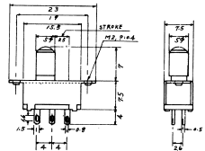
B15780 SLIDE SWITCH (2P4T)
