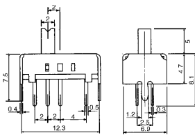
B15810 SLIDE SWITCH (4P3T)
