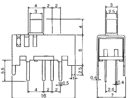
B15840 SLIDE SWITCH (8P3T)
