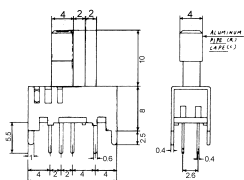
B15850 SLIDE SWITCH (8P4T)
