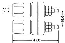
K2102 DOUBLE BINDING POST K2103 (GOLD PLATED)
