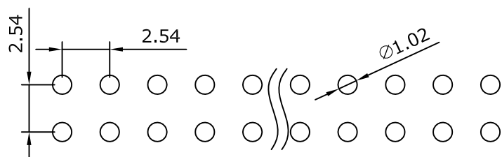
Recommended PCB Layout (PCB TOLERANCE \pm 0.05 )
