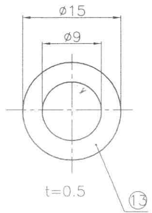
Spring 1PC
