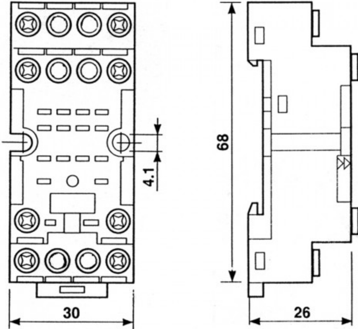
ZDV2 - two pole
