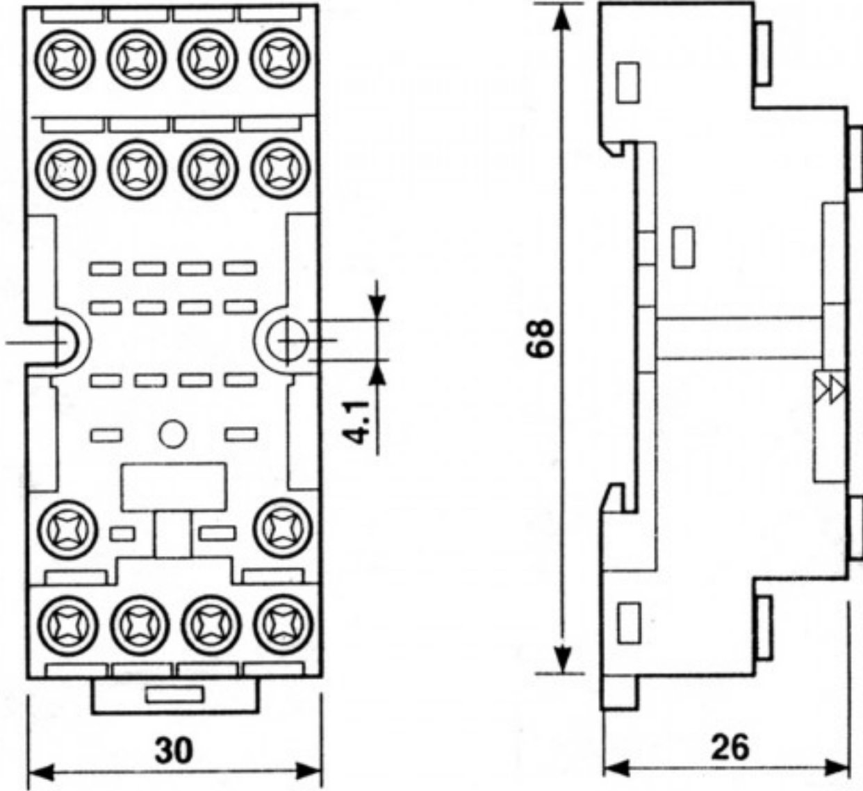
ZDV4 - four pole
