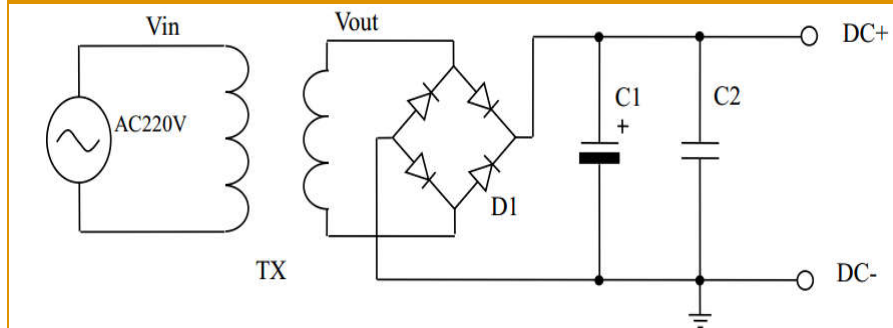
With linear power schematic
