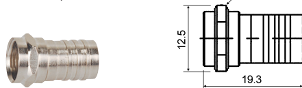
M5608 F male crimp type (RG59U/5C2V)
