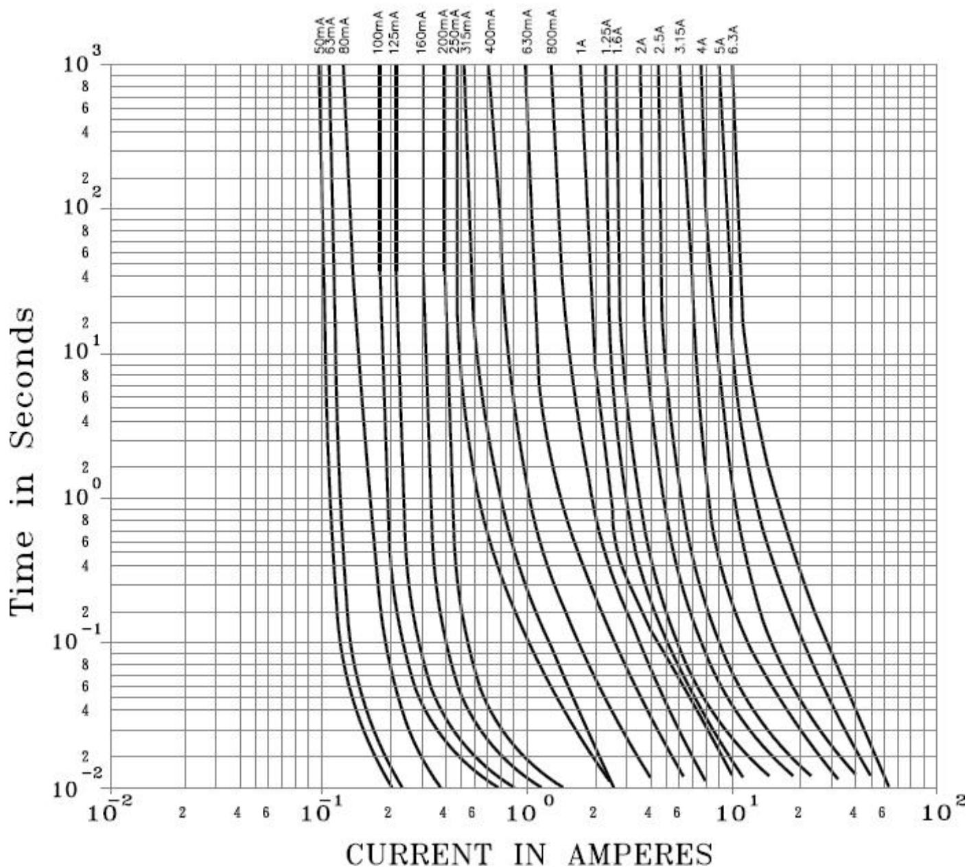
Average Time Current Curves : MEF
