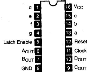
NTE74C925 16-Lead DIP, See Diag. 249 4-Digit Counter */Multiplexed Seven-Segment Output Driver
