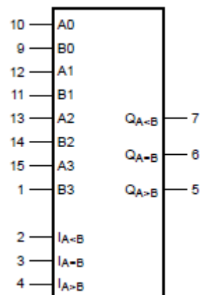
Figure 1. Logic symbol
