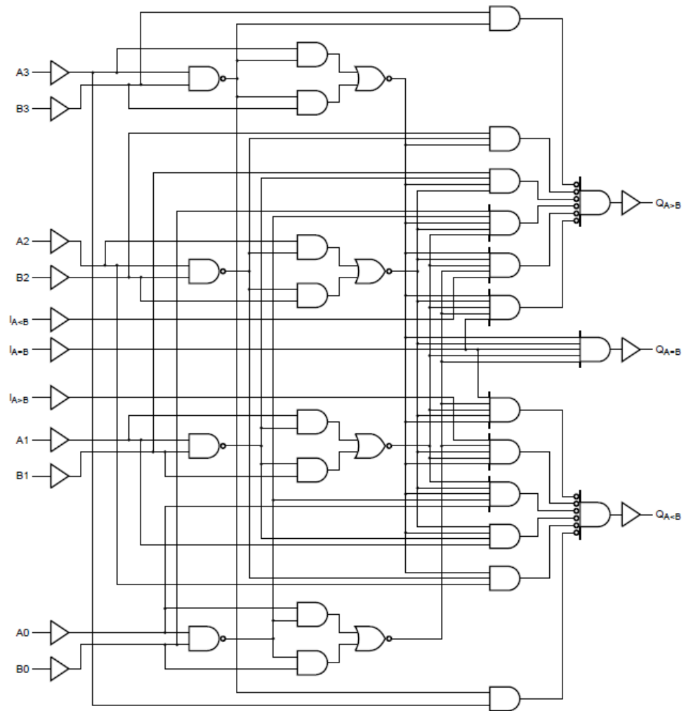
Figure 4. Logic diagram
